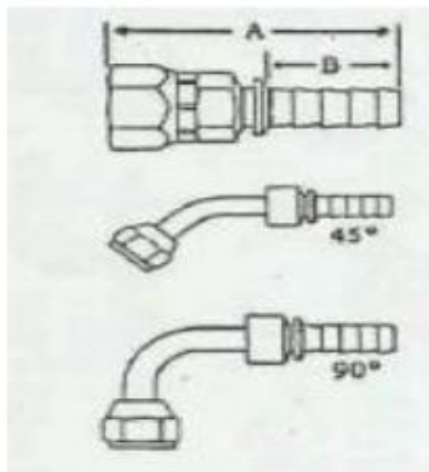
B.S.P FEMALE SWIVEL ASSEMBLY WITH FERRULE : E2A , E2T , M3
